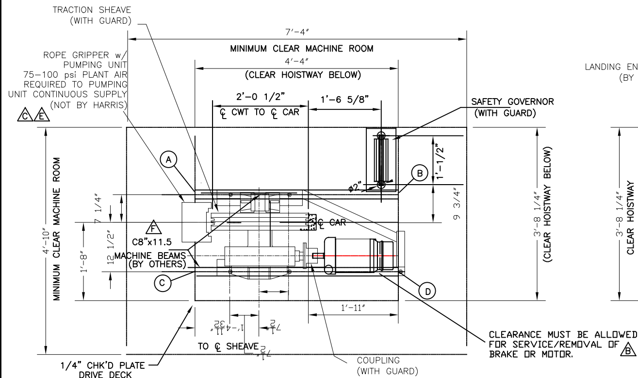
DRIVE LEVEL PLAN
