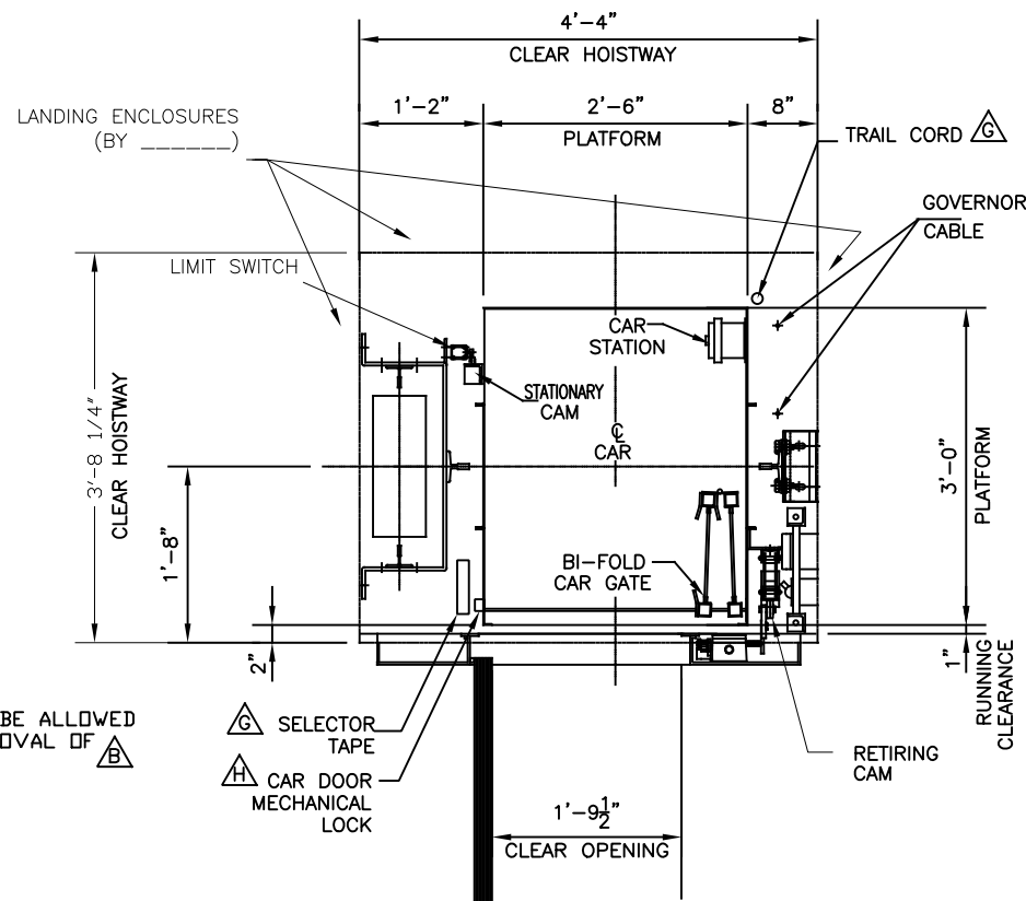
TYPICAL INTERMEDIATE LANDING PLAN
