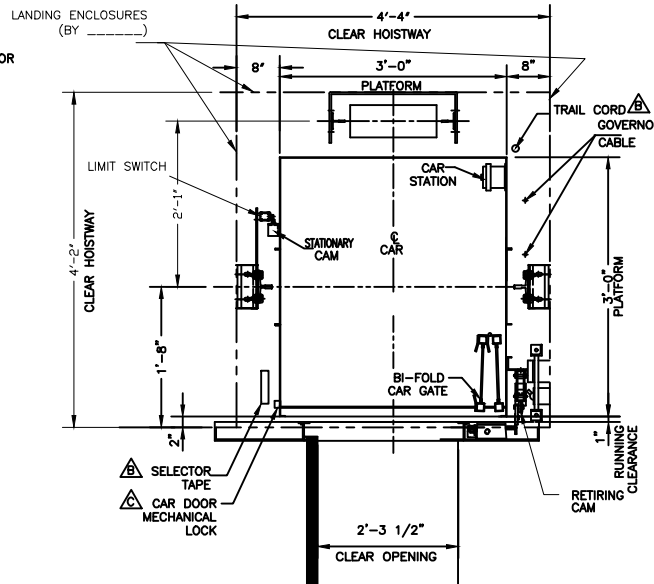
TYPICAL INTERMEDIATE LANDING PLAN
