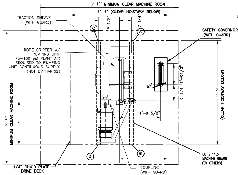
DRIVE LEVEL PLAN (NOT TO SCALE)
