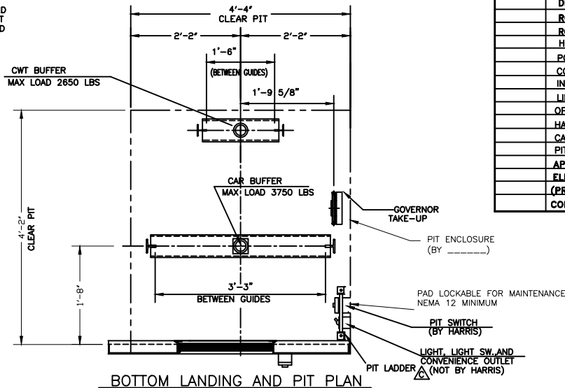
BOTTOM LANDING AND PIT PLAN
