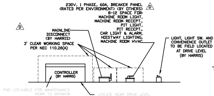
DRIVE LEVEL PLAN (NOT TO SCALE)
