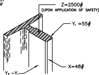
CAR GUIDE RAIL FORCES (CWT. RAIL FORCES NEGLIGIBLE)
