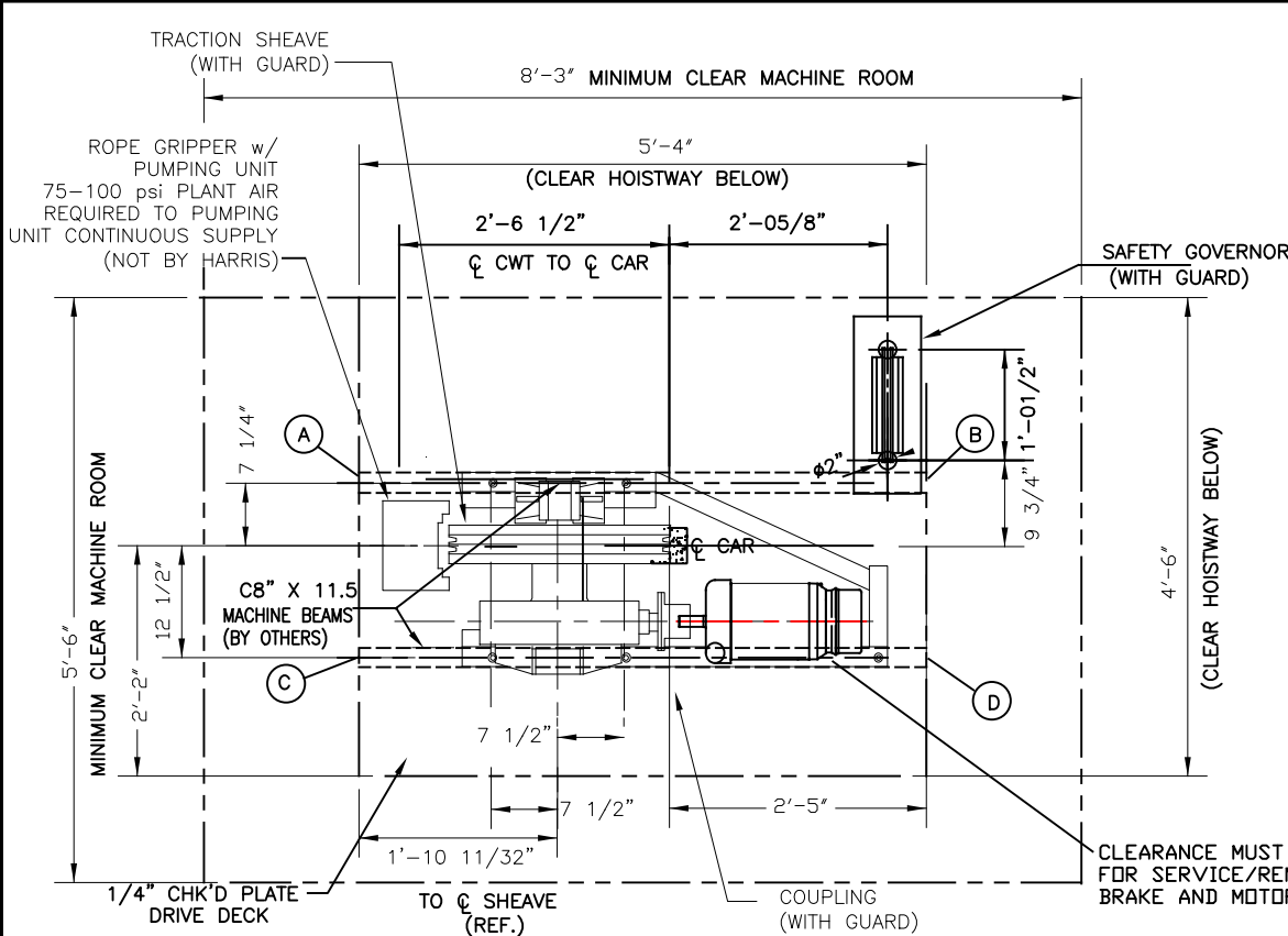
DRIVE LEVEL PLAN
