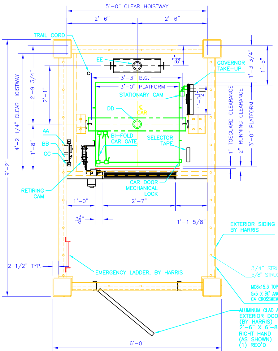
BOTTOM LANDING AND PIT PLAN
