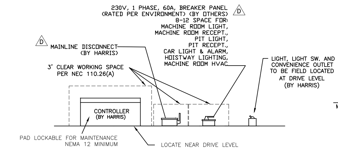
DRIVE LEVEL PLAN (NOT TO SCALE)
