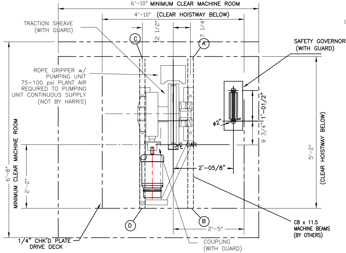
DRIVE LEVEL PLAN (NOT TO SCALE)
