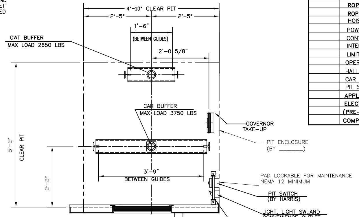
BOTTOM LANDING AND PIT PLAN
