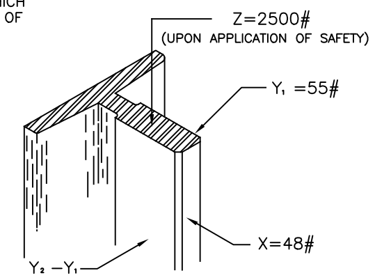
CAR GUIDE RAIL FORCES (CWT. RAIL FORCES NEGLIGIBLE)
