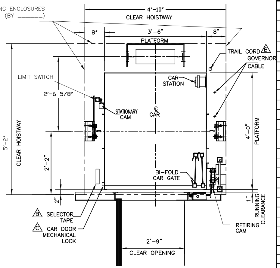
TYPICAL INTERMEDIATE LANDING PLAN
