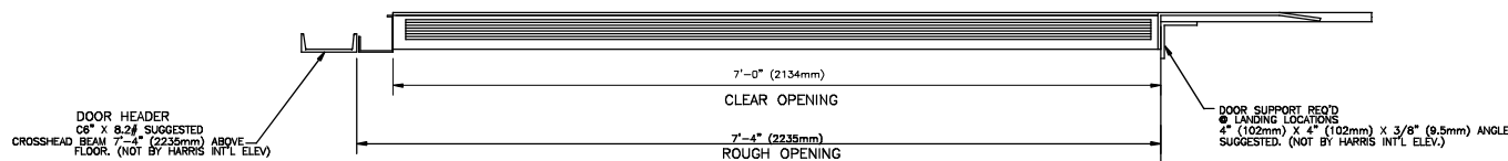
HOISTWAY ENTRANCE ELEVATION
