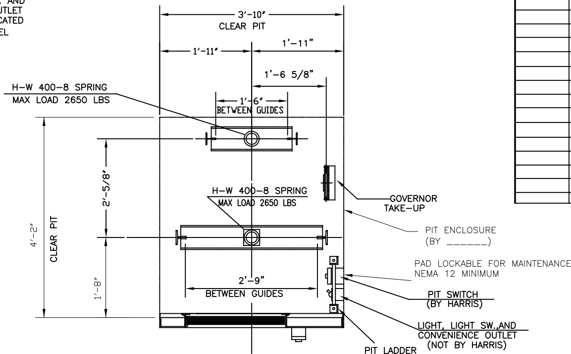
BOTTOM LANDING AND PIT PLAN
