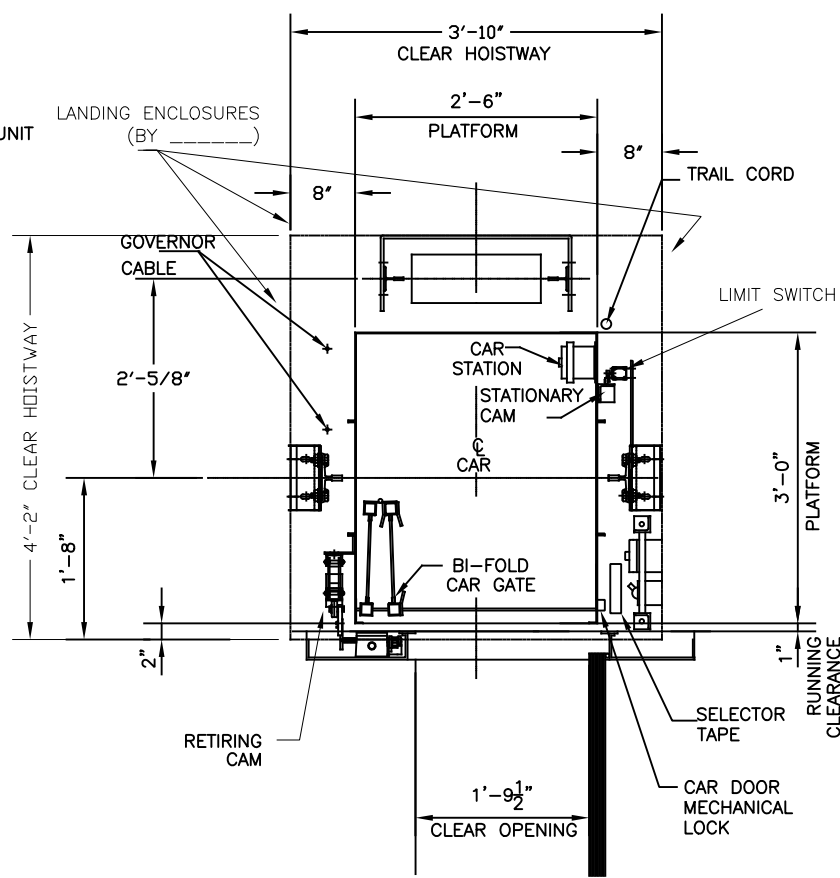
TYPICAL INTERMEDIATE LANDING PLAN
